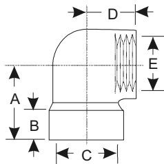
90° Adapter Elbow
